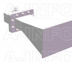
LB-340-10-C-7/16FSP Standard Gain Horn Antenna 2.2-3.3GHz 10dB Gain 7/16(DIN) Female
